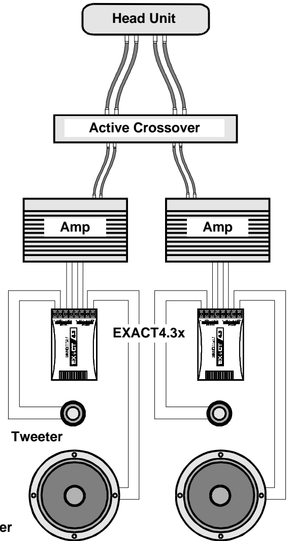
Figure 10 Active/Passive Bi-Amp
